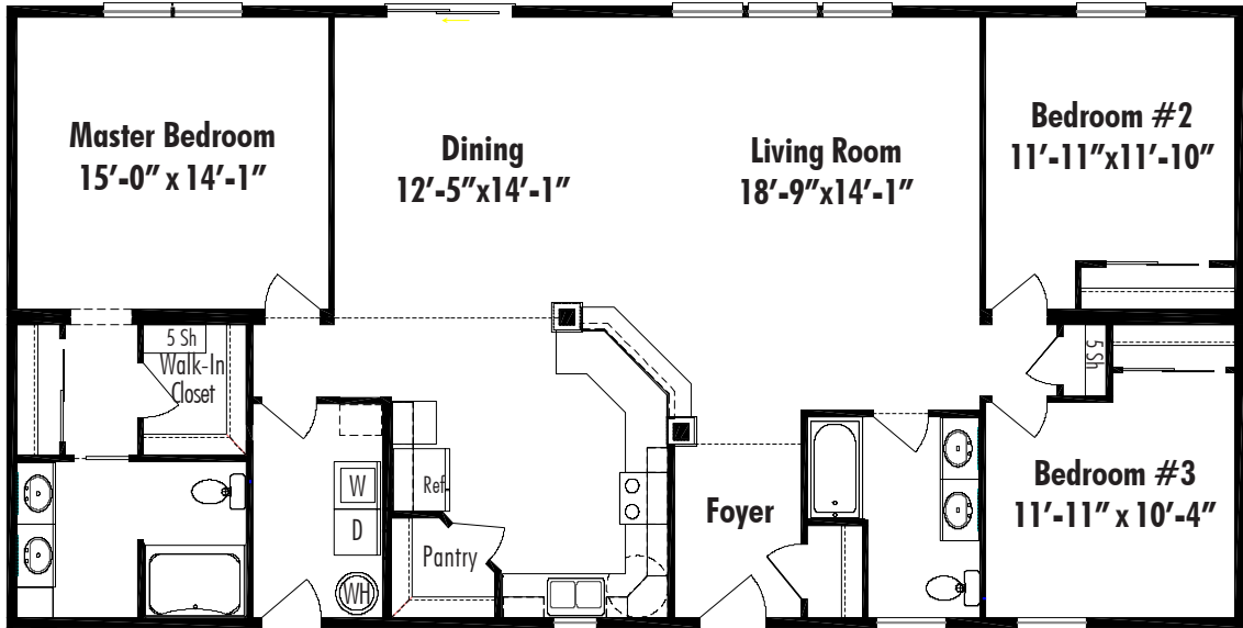
Anderson A Crawl Space 30' x 60', 1800 Sq. Ft. Living Area
